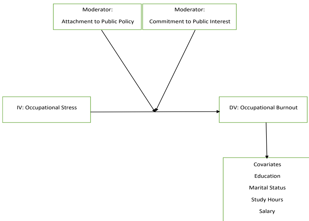
Figure 1: Schematic Presentation of Research Plan
